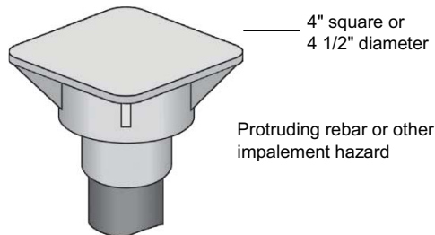
Illustration 2 | Protective Covers
